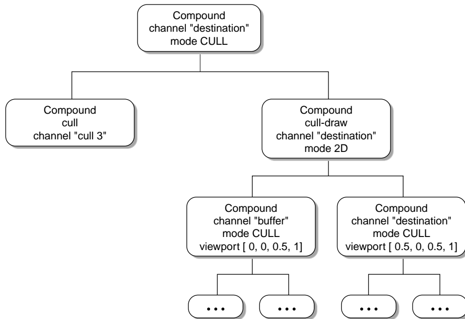
Figure 4-3 Compound Tree for 2D Decomposition and Multilevel Culling
