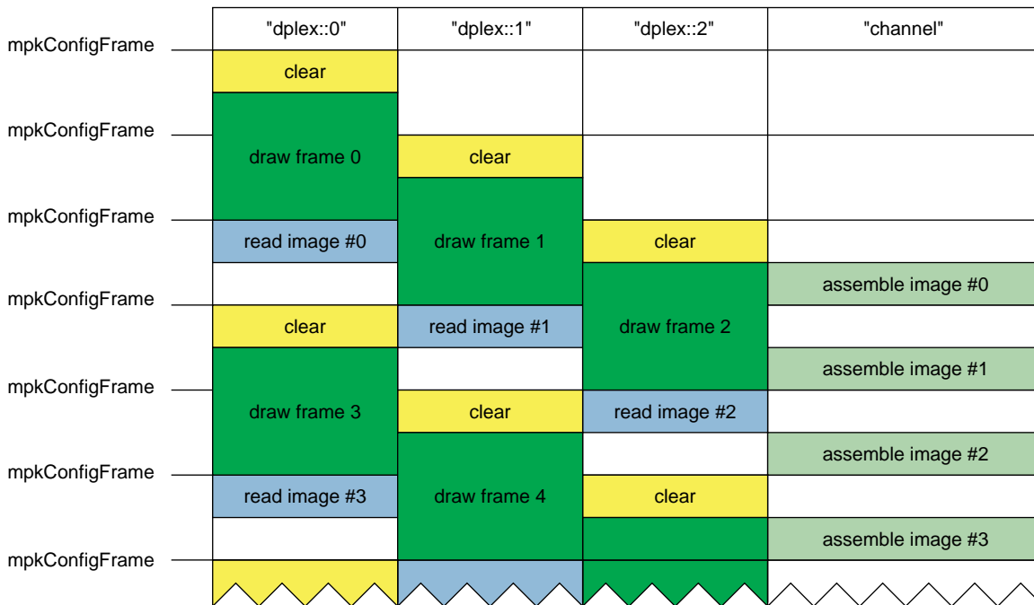
Figure 3-12 The Execution of a DPLEX Compound
