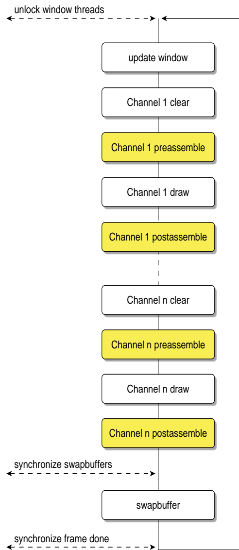
Figure 3-22 A Detailed Window Update
